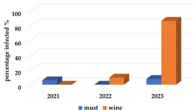
Figure 3. The dynamics of B. bruxellensis infection of musts and wines during three years of observation in the micro-winery. B. bruxellensis content was monitored in the wines produced in the micro-winery at different stages of wine-making.
