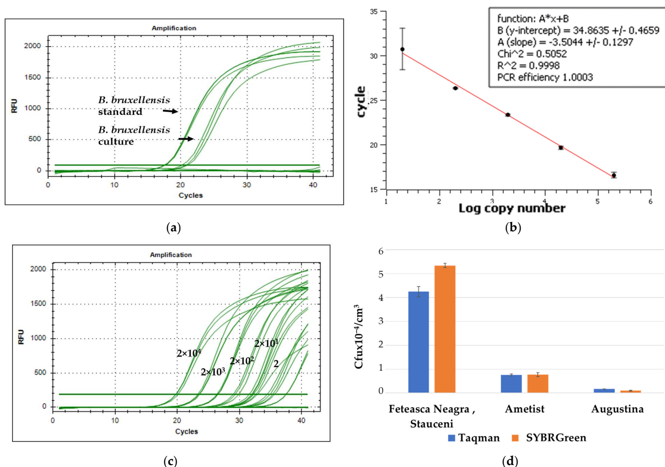
Figure 1. Validation of the primers for Brettanomyces detection and quantification. (a) Primer specificity of primers p35–p36. The amplification is observed only in the samples with B. bruxellensis standard DNA or culture DNA. (b) Standard curve for primers p35–p36. (c) LOD and LOQ of the primer pair p35–p36. (d) The results of quantification of B. bruxellensis by Taqman commercial kit and SYBR with home-designed primers.
