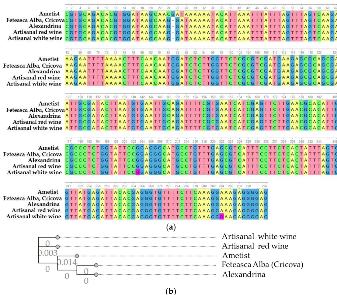
Figure 4. ITS1-ITS4 nucleotide sequences from individual B. bruxellensis isolates from artisanal wines and wines from micro-winery. (a) Alignment; (b) dendrogram of similarities. Different colours indicate different nucleotide bases.
