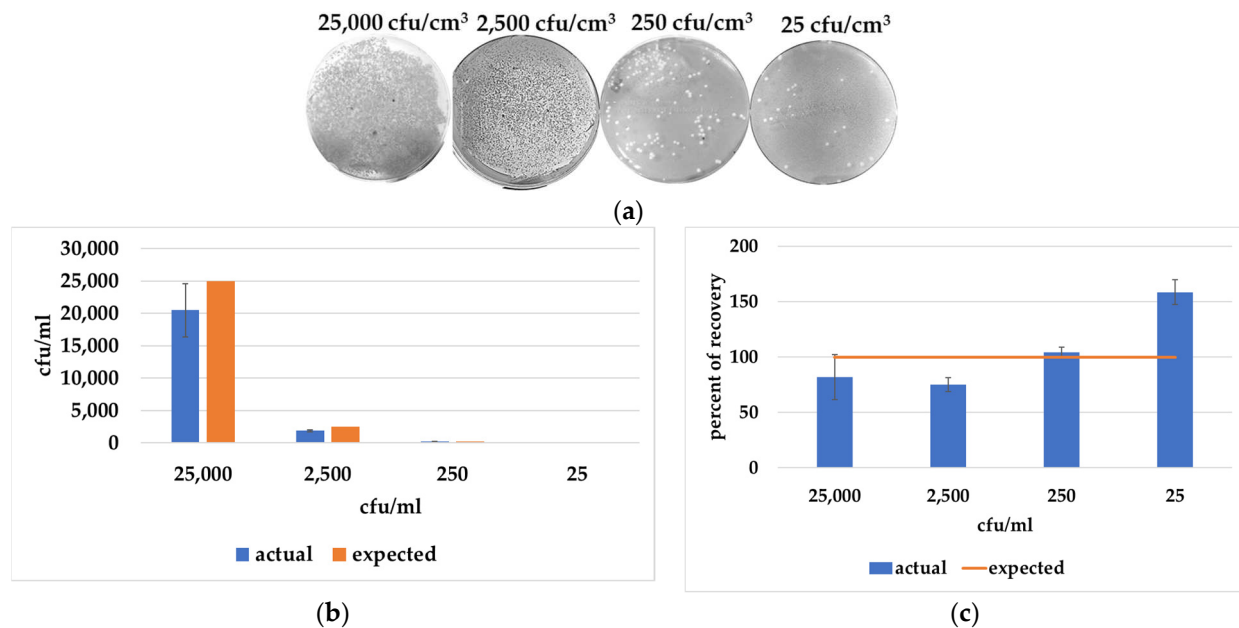
Figure 2. The quantification of B. bruxellensis in artificially infected sterile wine by colony count (a) and SYBR-based real-time PCR calculated in cfu/cm 3 (b) and percent of recovery (c).
