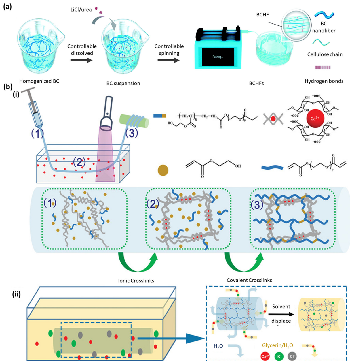
Fig. 6 Fabrication procedure of hydrogel-based optoelectronic fibers. (a) Wet spinning procedure of BCHFs using the nanofiber-rich BC suspension as a spinning solution and water as a coagulating bath. A dense hydrogen bond was formed between cellulose nanofibers and molecular chains leading to continuous BCHFs. Reproduced with permission from ref. 213, Copyright © 2021 Royal Society of Chemistry. (b) (i) Wet spinning process of an organohydrogel with the evolution of polymeric networks at different stages of the spinning process. (1), (2) and (3) represent the structural evolution at different stages during spinning including (1) spinning solution, (2) ion-crosslinked fiber, and (3) hybrid crosslinked fiber. (ii) Preparation of organohydrogel fibers by the solvent displacement method. Reproduced with permission from ref. 215, Copyright © 2020 John Wiley & Sons, Inc.
