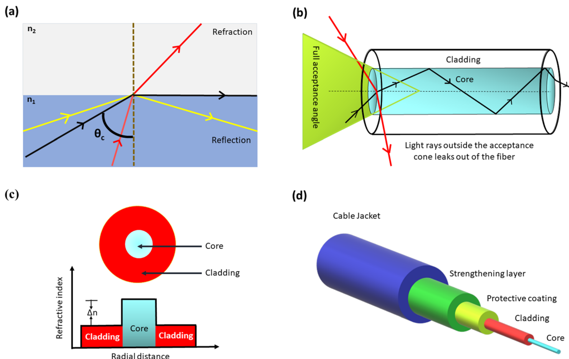
Fig. 3 Guiding mechanisms of an optical fiber. (a) Total internal reflection at the interphase of two different media, (b) acceptance angle of an optical fiber, (c) refractive index profile of a step-index optical fiber and (d) optical fiber structure with protective layers.
