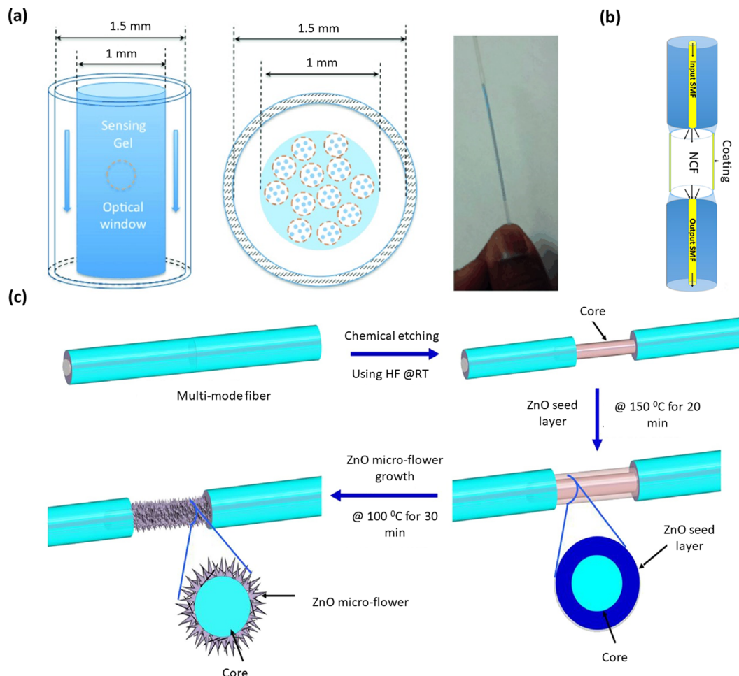
Fig. 10 Hydrogel-based optical fiber sensors for pH monitoring. (a) Demonstration of a capillary optode including nanocapsule loaded sensing gel at the core. Reproduced with permission from ref. 305, Copyright © 2015 John Wiley & Sons, Inc. (b) Illustration of the SMF-no core-SMF fiber coated with SiO 2 embedded PVA/PAA. Reproduced with permission from ref. 313, Copyright © 2021 The Optical Society. (c) Fiber optic probe fabrication through ZnO microflower growth. Reproduced with permission from ref. 304, Copyright © 2018 Elsevier Ltd.
