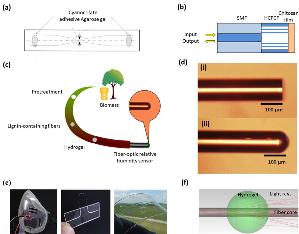
Fig. 11 Hydrogel-based optical fiber sensors for humidity sensing. (a) Schematic of a biconically tapered optical fiber. Reproduced with permission from ref. 325, Copyright © 2000 Elsevier Ltd. (b) FPI-based sensor with chitosan hydrogel. Reproduced with permission from ref. 327, Copyright © 2015 Taylor & Francis Ltd. (c) Preparation of hydrogel from renewable biomass for fiber optic humidity sensor. (d) Microscopic images of (i) a cut fiber end and (ii) an optical fiber sensor with cellulose film at the tip. (c and d) Reproduced with permission from ref. 26, Copyright © 2021 Elsevier Ltd. (e) Practical application of the U-bend fiber optic RH sensor (sensor implemented oxygen mask, cladding stripped plastic optical fiber U-bend sensor, and a polymer bare fiber laminated flexible device between two PMMA substrate layers). Reproduced from ref. 331, Copyright © 2017 The Author. Published by MDPI. (f) Illustration of the hydrogel sphere-based fiber optic sensor. Reproduced with permission from ref. 339, Copyright © 2015 Elsevier Ltd.
