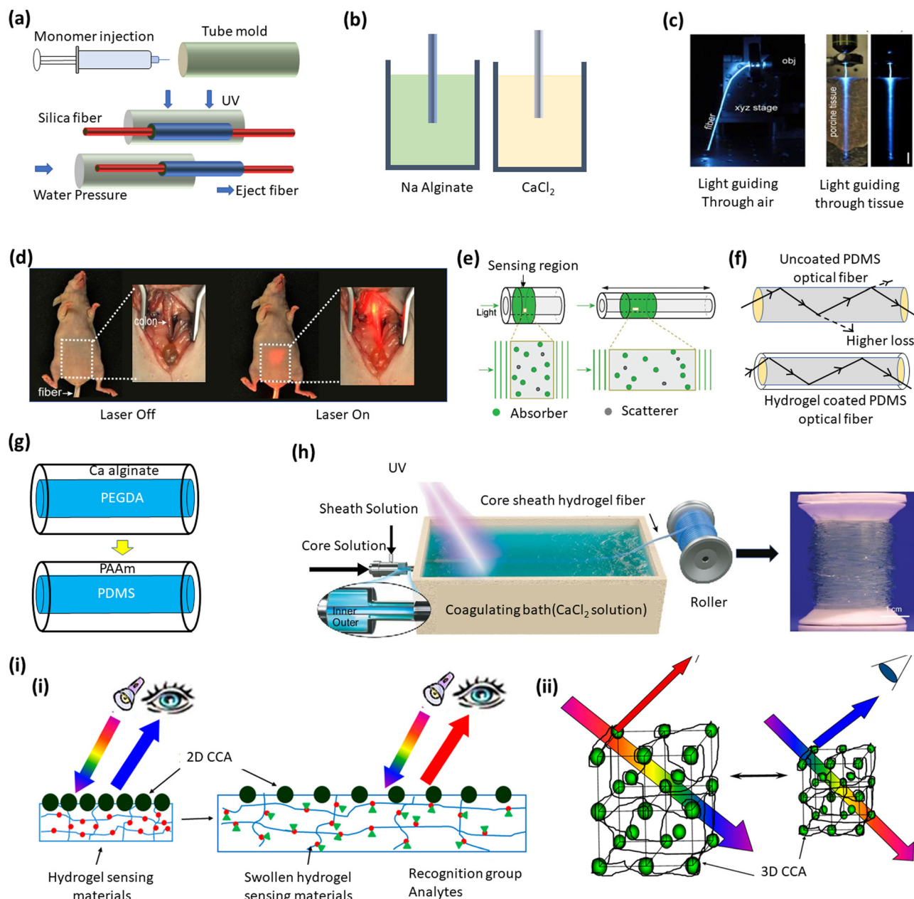
Fig. 5 Hydrogel-based pure optical waveguides. (a) Fabrication procedure of the hydrogel optical fiber core, (b) Ca alginate deposition on a bare fiber core, (c) demonstration of blue light (492 nm) guiding through the hydrogel optical fiber between two thin porcine tissue slices, (d) light guidance from rectum to the colon of an anesthetized mouse, confirmed by abdominal laparotomy. (c and d) Reproduced with permission from ref. 34, Copyright © 2015 John Wiley & Sons, Inc. (e) Hydrogel-based strain sensor. Reproduced with permission from ref. 73, Copyright © 2016 John Wiley & Sons, Inc. (f) Hydrogel-coated PDMS core optical fiber with increased light confinement in the core region, (g) alginate coating replaced by PAAm clad PDMS structure for lower loss, (h) continuous hydrogel optical fiber production through a dynamic wet spinning process (ILDWS) and collected fibers around a spool. Reproduced from ref. 201, Copyright © 2020 The Author. Published by Oxford University Press. (i) Hydrogel based (i) 2D and (ii) 3D photonic crystals by attaching 2D or 3D CCAs onto a hydrogel containing functionalized recognition groups. Reproduced with permission from ref. 44, Copyright © 2015 American Chemical Society.
