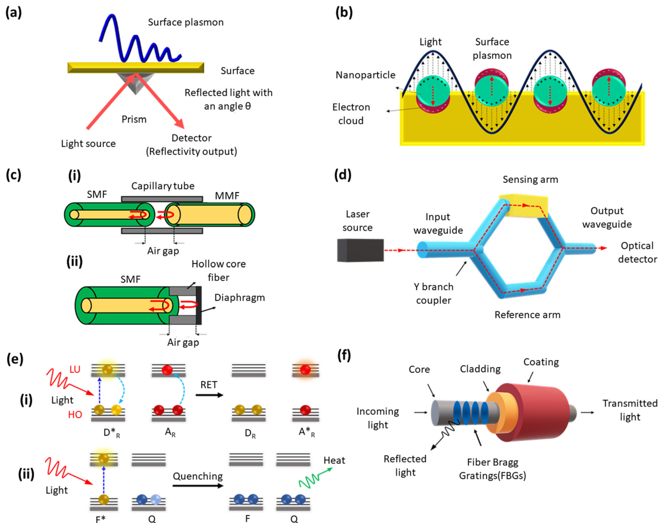
Fig. 4 Sensing principles of hydrogel-based optical fibers: (a) surface plasmon resonance (SPR), (b) localized surface plasmon resonance (LSPR), (c) Fabry–Perot cavities: (i) fiber air gap-based cavity and (ii) diaphragm based cavity, (d) Mach–Zehnder interferometer-based sensor, (e) fluorescence sensing mechanisms: (i) resonance energy transfer (RET) mechanism and (ii) quenching mechanism (F: fluorophore, Q: quencher) and (f) Fiber–Bragg grating sensor.
