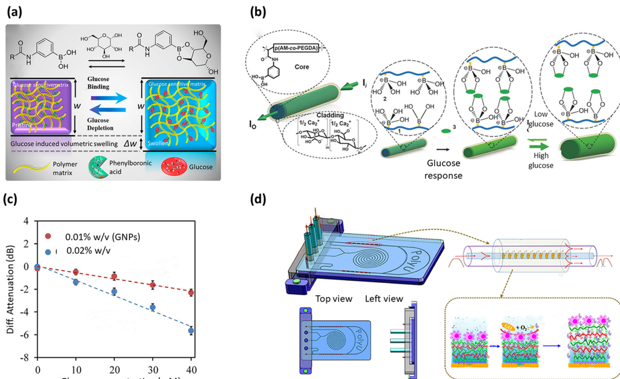
Fig. 9 Hydrogel-based optical fiber sensors for glucose sensing. (a) Glucose-binding process and volumetric shift of the hydrogel due to the addition or removal of glucose. Reproduced with permission from ref. 295, Copyright © 2018 American Chemical Society. (b) 3-APBA functionalized hydrogel matrix (1 → polyacrylamide hydrogel crosslinked with PEG, 2 → charged tetrahedral state of 3-APBA, 3 → glucose) and its response to glucose. Reproduced from ref. 76, Copyright © 2017 The Author. Published by John Wiley & Sons, Inc. (c) Differential light attenuation (at 528 and 700 nm) for different glucose concentrations of 0.01 wt% and 0.02 wt% gold nanoparticle doping. Reproduced with permission from ref. 137, Copyright © 2021 Walter de Gruyter GmbH. (d) Design of a microfluidic chip integrated with an optical fiber glucose biosensor with the mode coupling and optical resonance of the sensor and the glucose sensing and signal enhancing mechanism of the film. Reproduced with permission from ref. 301 Copyright © 2016 The Optical Society.
