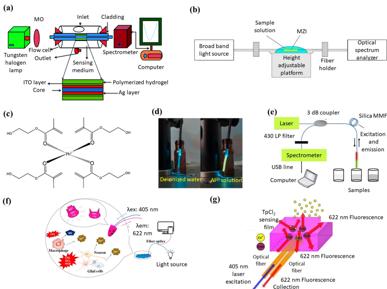
Fig. 12 Hydrogel-based optical fiber sensors for ion sensing. (a) Schematic representation of the experimental design. Reproduced with permission from ref. 341, Copyright © 2014 Royal Society of Chemistry. (b) Experimental design of the sensing equipment. Reproduced with permission from ref. 262, Copyright © 2014 Elsevier Ltd. (c) Interaction between \text{Pb}^{2+} ions and probe molecules. Reproduced with permission from ref. 161, Copyright © 2022 Elsevier Ltd. (d) Change of fluorescence intensity after \text{Al}^{3+} immersion. Reproduced with permission from ref. 349, Copyright © 2021 Elsevier Ltd. (e) Experimental setup for the ratiometric sensing of the probe molecule. Reproduced with permission from ref. 74, Copyright © 2018 Elsevier Ltd. (f) Mechanism of sensing with double fibers. Reproduced with permission from ref. 352, Copyright © 2020 Elsevier Ltd. (g) The working mechanism of the sensing film with two fibers. Reproduced with permission from ref. 355, Copyright © 2015 Elsevier Ltd.
