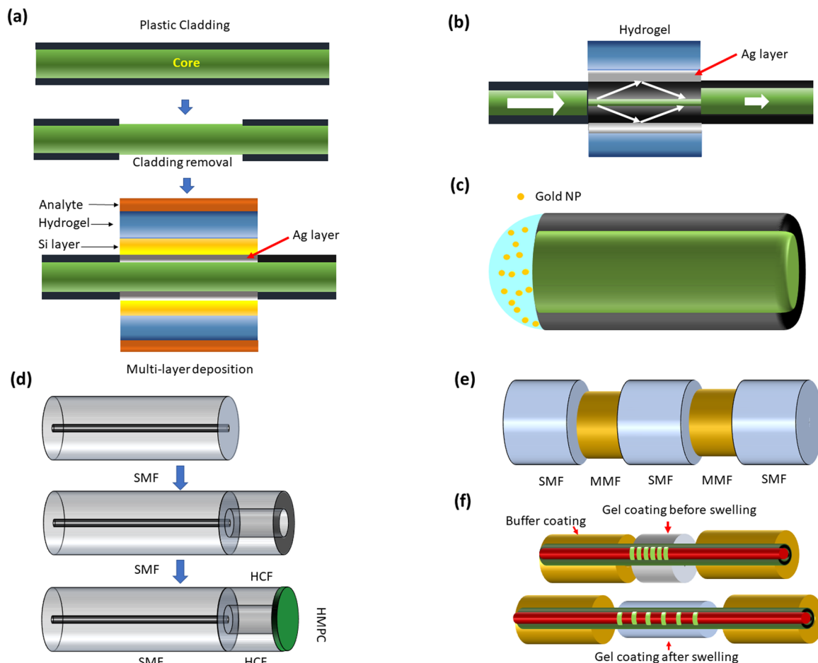
Fig. 7 Schematic illustrations for fabrication procedures of various hydrogel-based optical fiber sensors: (a) hydrogel-based SPR sensor. Reproduced with permission from ref. 220, Copyright © 2012 Elsevier Ltd. (b) Spliced MMF-SMF-MMF structure SPR sensor. Reproduced with permission from ref. 35, Copyright © 2018 Elsevier Ltd. (c) LSPR-based hydrogel fiber optic sensor with a functionalized tip. Reproduced from ref. 235, Copyright © 2017 The Author. Published by MDPI. (d) SMF-HCF-HMPA-based Fabry-Perot interferometry-based sensor. Reproduced with permission from ref. 147, Copyright © 2019 Elsevier Ltd. (e) SMF-MMF-SMF-MMF-SMF spliced structure for the Mach-Zehnder interferometry-based fiber optic sensor. Reproduced with permission from ref. 263 Copyright © 2019 The Optical Society. (f) Bragg grating-based hydrogel fiber optic sensor. Reproduced with permission from ref. 268, Copyright © 2016 SPIE.
