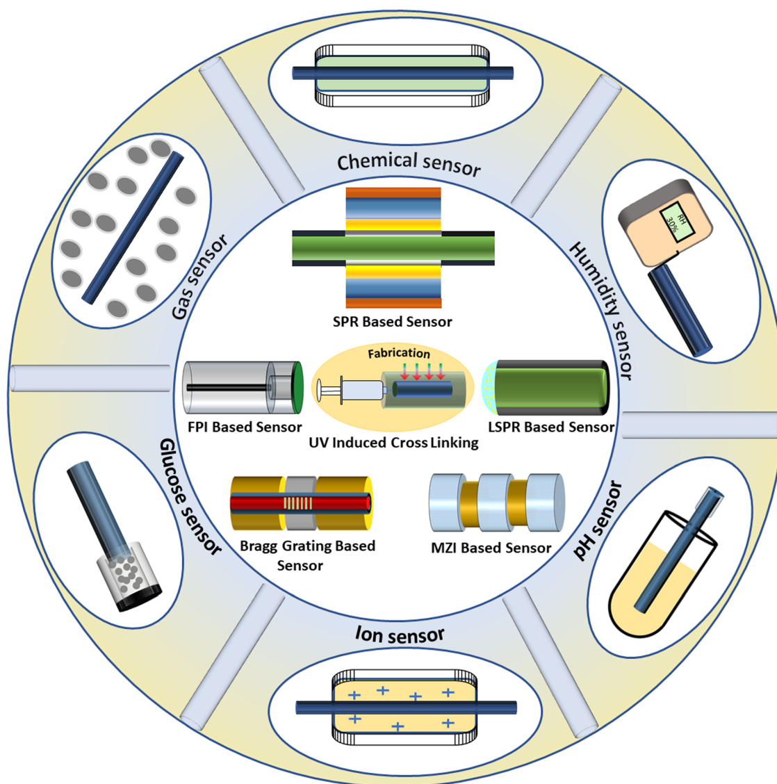
Fig. 1 Illustration of the fabrication methods of pure optical waveguides and optical sensors (SPR, LSPR, FPI, MZI and Bragg grating based sensors) and the major applications (glucose, pH, humidity, ion, gas and chemical sensing) of hydrogel-integrated optical fiber sensors.
