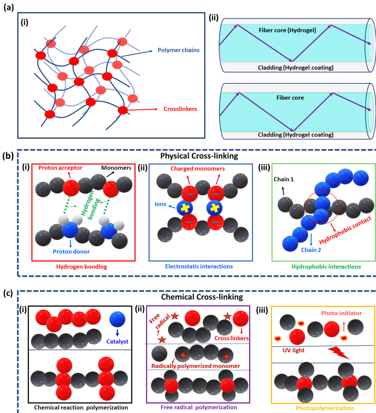
Fig. 2 Structure and synthesis of hydrogels. (a) Hydrogel formation for optical fiber applications: (i) crosslinking of polymer chains for hydrogel formation and (ii) usage of hydrogels as the core/cladding (above) and cladding (below) of an optical fiber. (b) Physically crosslinking methods used for formation of a hydrogel: (i) cross-linking of polymeric chains via hydrogen bonding to form a hydrogel, (ii) cross-linking via electrostatic interactions between charged polymeric chains and ions, and (iii) cross-linking through hydrophobic interactions between polymeric chains. (c) Hydrogel formation by chemically crosslinking methods: (i) crosslinking of two polymers (black and red) using chemical reaction in the presence of a catalyst (blue), (ii) free radical polymerization of polymers (black) with crosslinkers (red) initiated by free radicals (stars), and (iii) polymerization of photosensitive monomers (black) with photo-initiators (red) under UV light.
