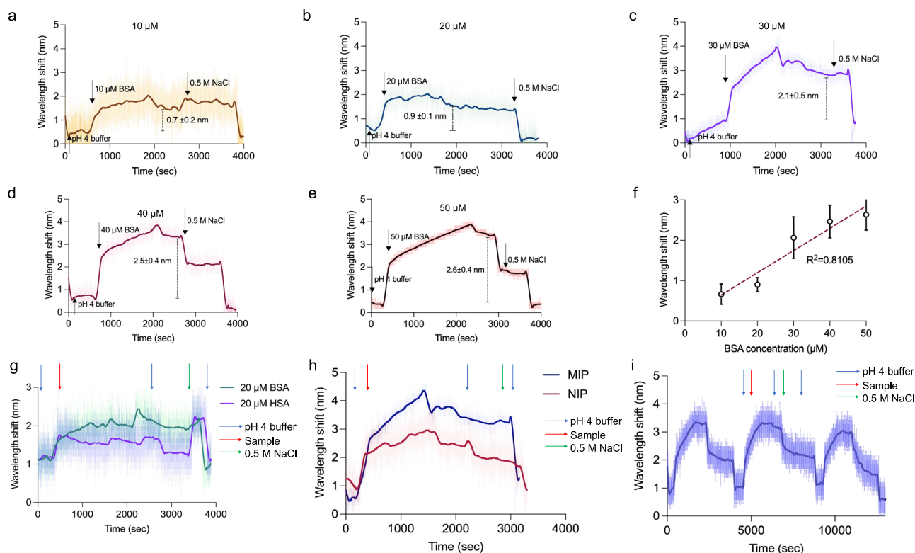
Fig. 7 | Binding studies. a–f The plots display the binding results of BSA protein solutions at different concentrations: a 10 \mu\text{M} , b 20 \mu\text{M} , c 30 \mu\text{M} , d 40 \mu\text{M} , and e 50 \mu\text{M} . f The calibration curve is plotted for evaluating the plasmonic signals upon the increments of protein concentrations. g As a selectivity analysis, the binding of BSA and HSA proteins is evaluated on the sensor modified with MIP nanoparticles. Wavelength shifts are collected in real-time data for BSA and HSA solutions at the same concentrations (20 \mu\text{M} for both protein solutions), and this plot states the selective binding of BSA protein to the MIPs. h Imprinting factor is evaluated
