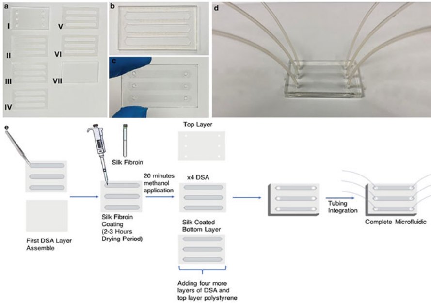
Fig. 1 All the components to fabricate microfluidic chips and the procedure of SF integration to the chips. (a) The chip consists of polystyrene materials (I, VII) and DSA films (II-VI). (b) Microchannels are formed with the first DSA first. (c) SF-coated microfluidic chip. (d) Full functional chip is finalized by tubing. (e) Schematic representation of all fabrication and modification steps
