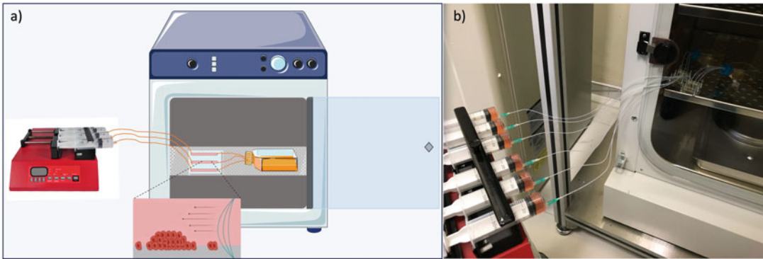
Fig. 2 A microfluidic chip operated with a syringe pump is employed to culture cells inside an incubator. (a) Schematic representation and (b) real experimental setup are exhibited. For scaling-up, the experiment can be operated with multiple channels of a chip and/or multiple microfluidic chips at the same time. In this representative experimental set, cell culture is performed in two separate microfluidic chips simultaneously
