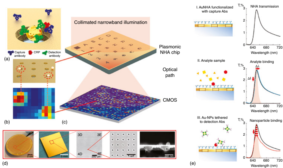
Figure 1.8 CRP detection via AuNP-enhanced plasmonic imager. (a) The schematic represents the capture of CRP (red) by an antibody (blue) on AuNHA and the detection of CRP by detection antibodies (green) tethered to AuNPs, respectively. (b) AuNPs create intensity dips (i.e. red spots) on captured image due to strong local suppression in the transmission. (c) Array labeling for accurate image processing and heatmap generation via CMOS camera for digital detection. (d) AuNHA wafer with 50 sensors. The plasmonic sensor surface is covered with AuNHAs. An image of microarray labels after patterning. The image of nanoholes ( D = 200\text{ nm} , P = 600\text{ nm} ) and the image of the nanohole containing AuNP are represented in the order from left to right. (e) (i) Transmission spectrum of the AuNHAs, (ii) peak position shift after the analyte binding, and (iii) local suppression after the binding of AuNPs to the AuNHA surface. Source: Reprinted with permission from Belushkin et al. [96]. © 2018, American Chemical Society.
